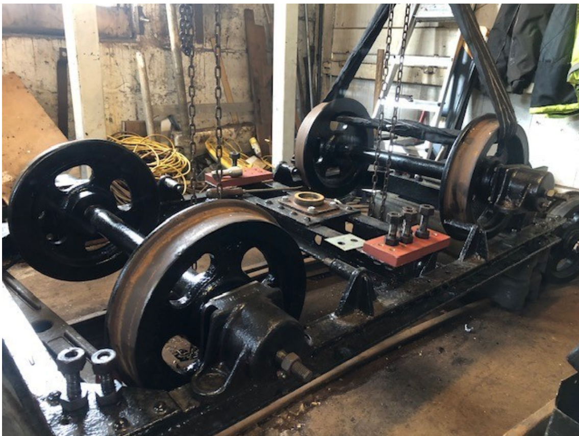
Wheelset nearing completion with new wheel bearings (photo Tina Brown)
